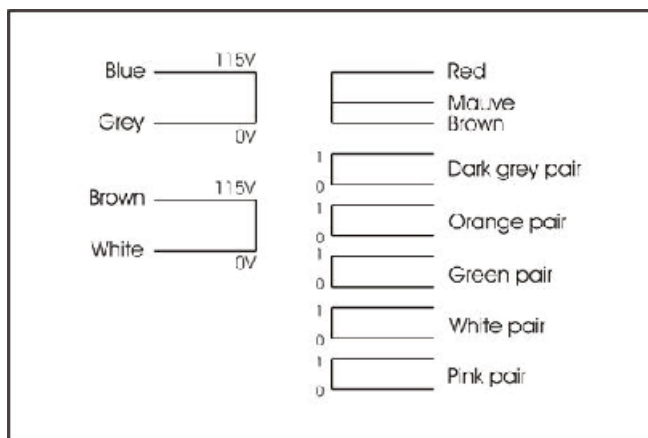
Figure 2. Mains transformer windings
